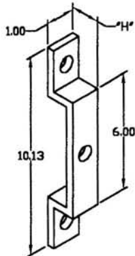
Mounting Bracket
