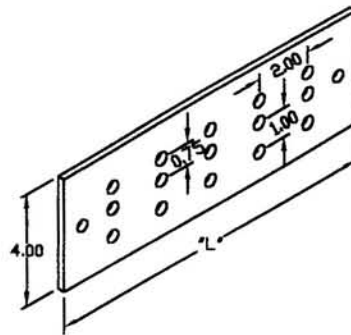
Plain Ground Bar
